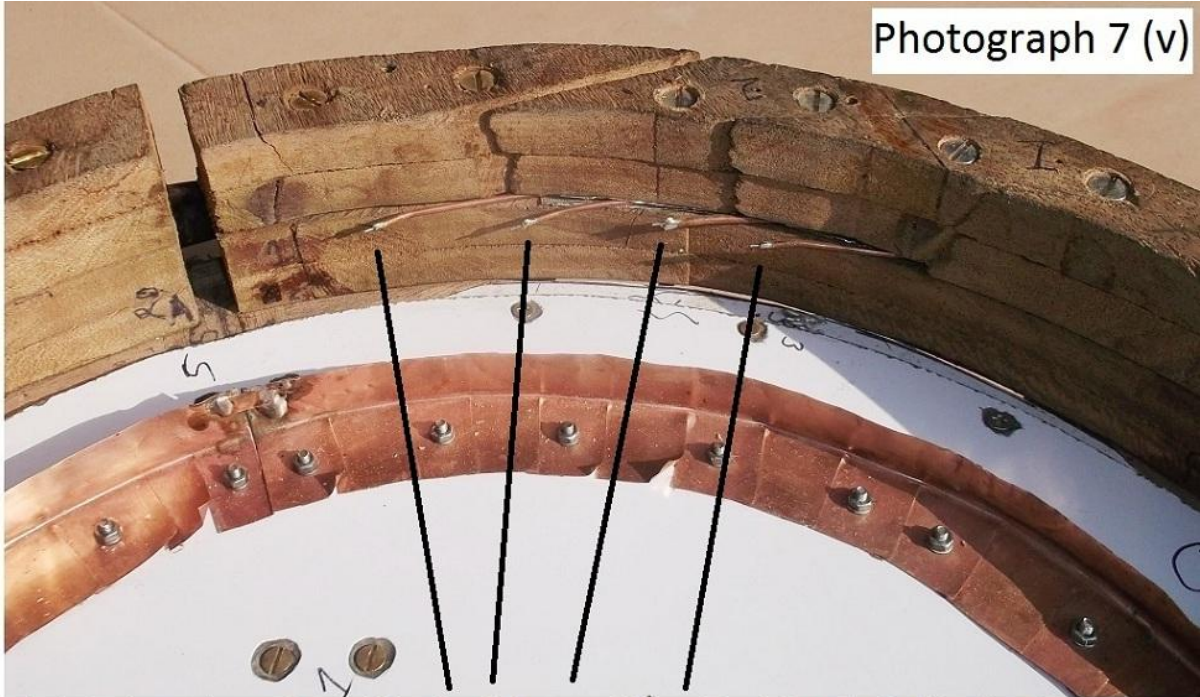
4 jets/nozzles placed in the Vapour/Gas Turbine to let in the Vapours of Working Fluid to hit against the Copper sheet fins of the Aluminium Wheel/Impeller .
