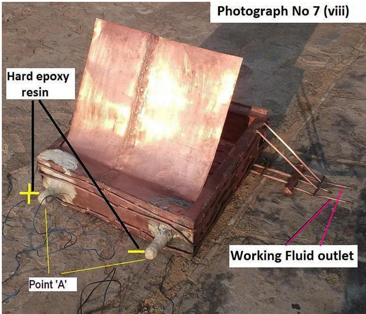
Turbine Box - view of Working Fluid outlet , positive and negative wires sealed with hard epoxy resin .
