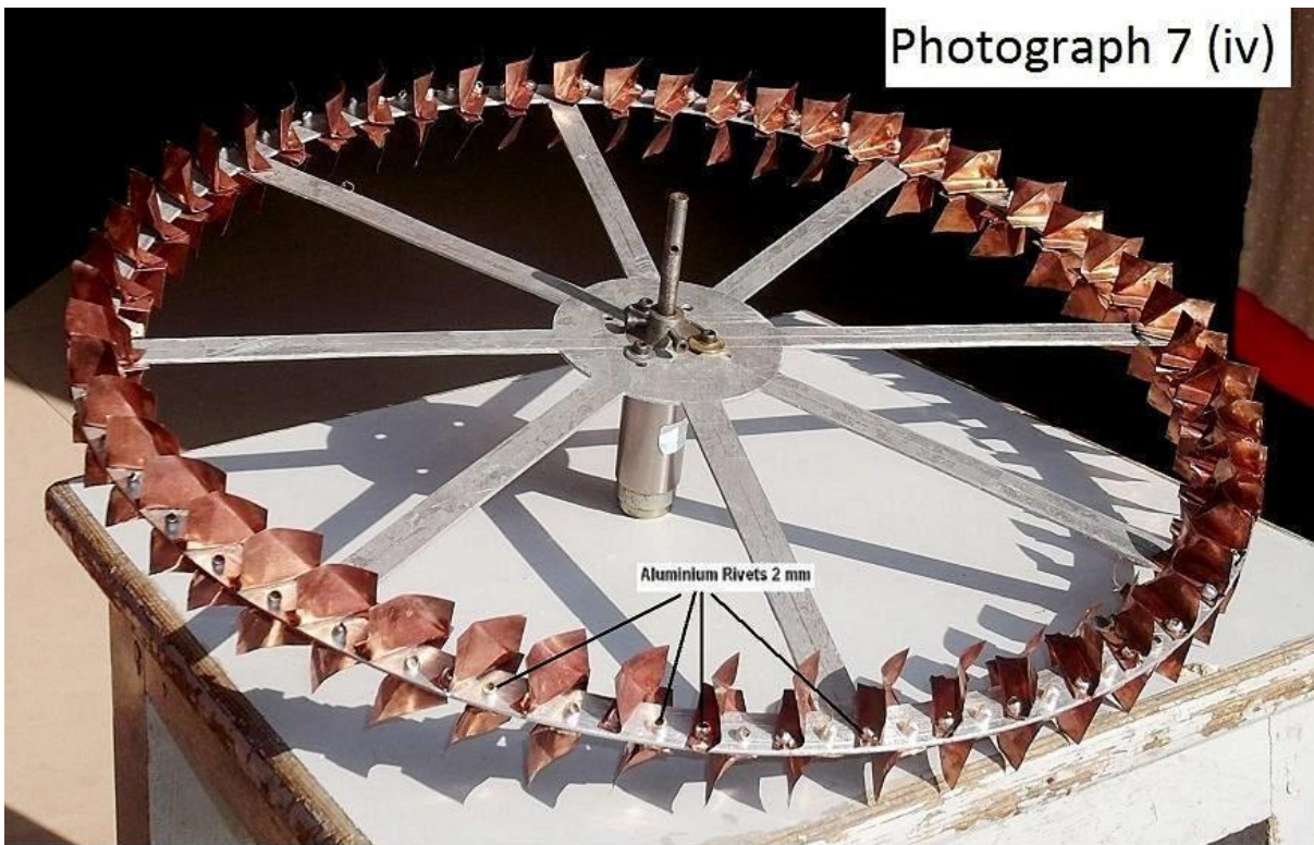
Aluminium Wheel/Impeller ( with attached Copper sheet fins ) with the Generator/Dynamo held in the centre by the holder ( made of mild-steel ) .
