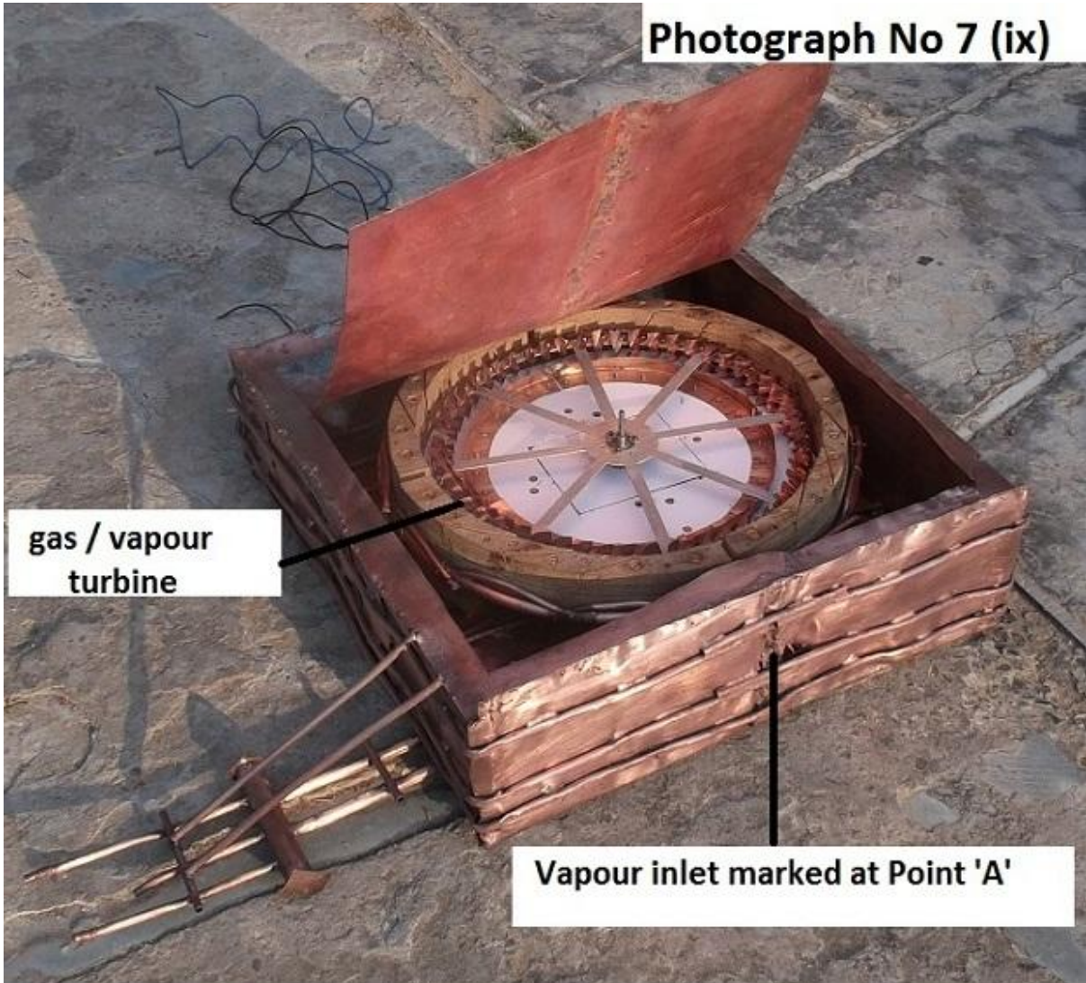
Turbine Box with Vapour/Gas Turbine placed inside . Vapour inlet marked at Point 'A'
